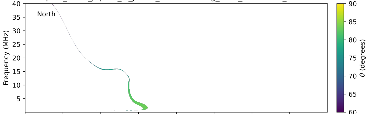
expres_earth_jupiter_io_jrm33_lossc-wid1deg_3kev_20280309_v11.cdf
