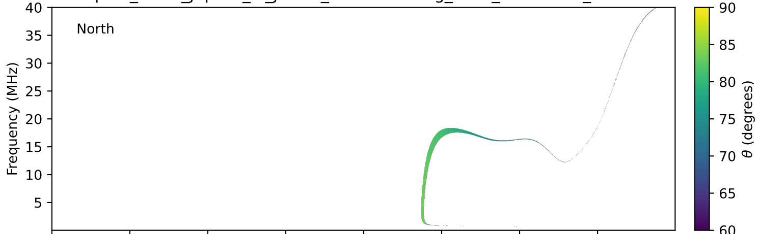
expres_earth_jupiter_io_jrm33_lossc-wid1deg_3kev_20280308_v11.cdf
