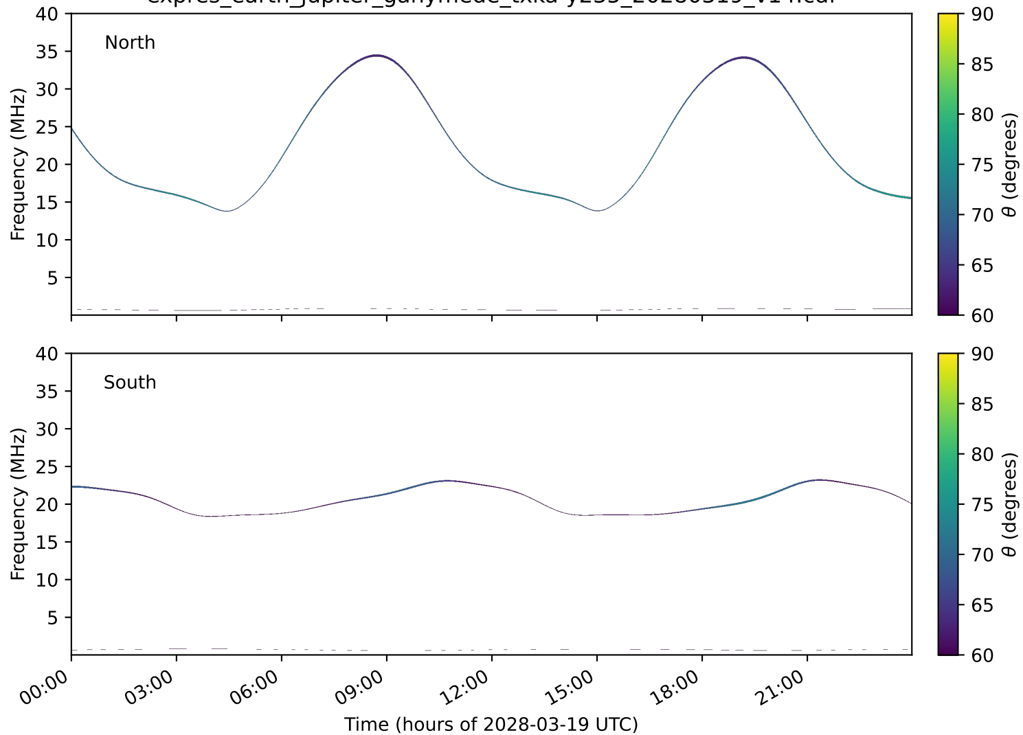
expres_earth_jupiter_ganymede_txka-y235_20280319_v14.cdf
