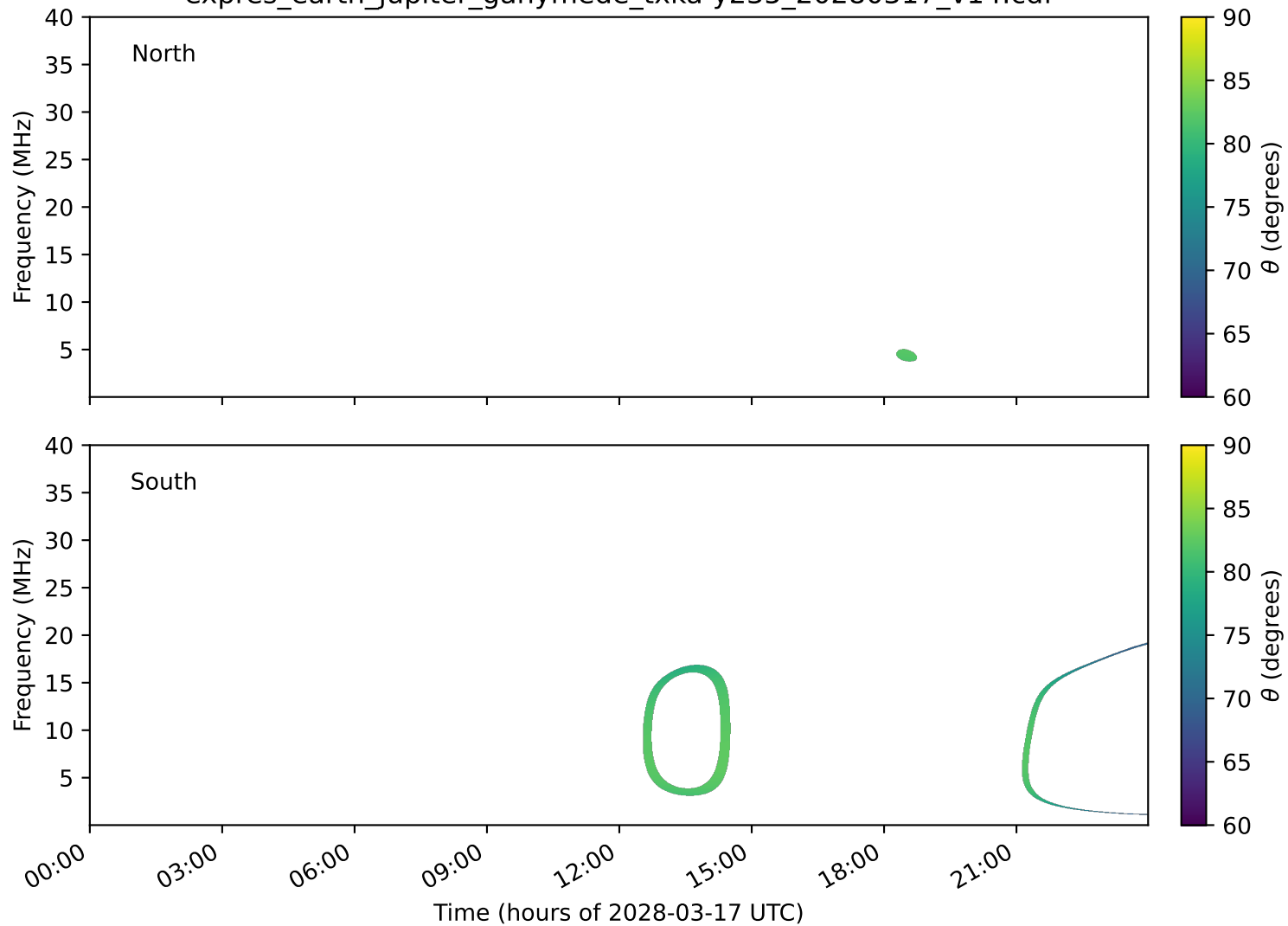
expres_earth_jupiter_ganymede_txka-y235_20280317_v14.cdf
