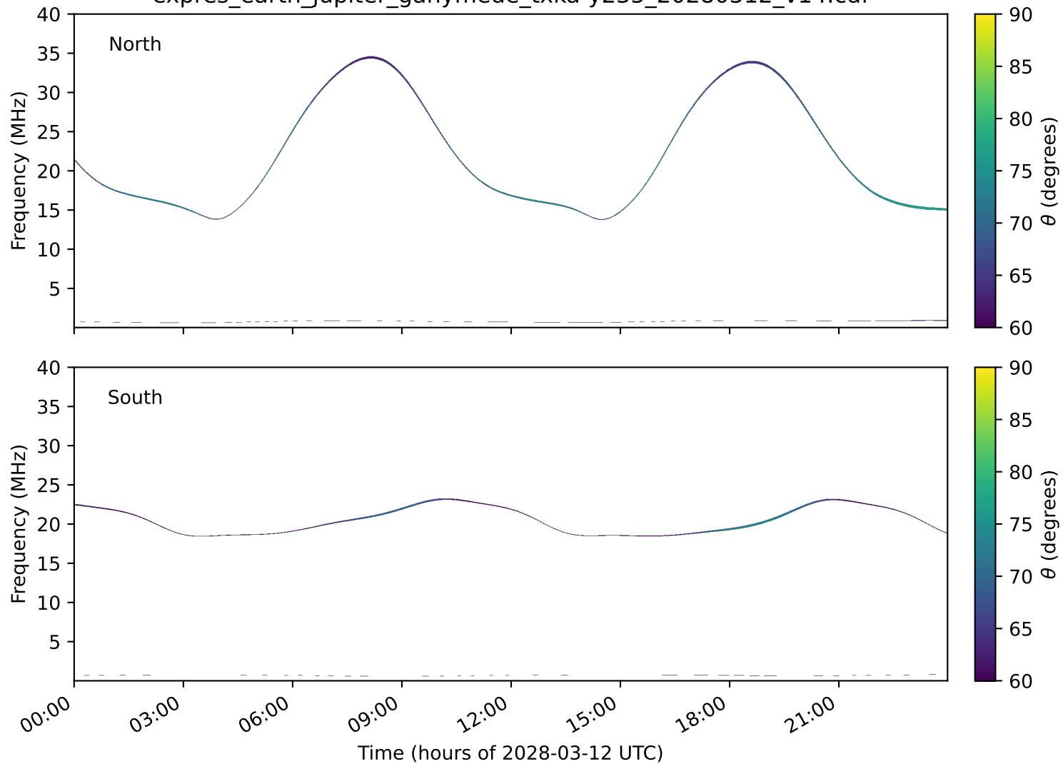
expres_earth_jupiter_ganymede_txka-y235_20280312_v14.cdf
