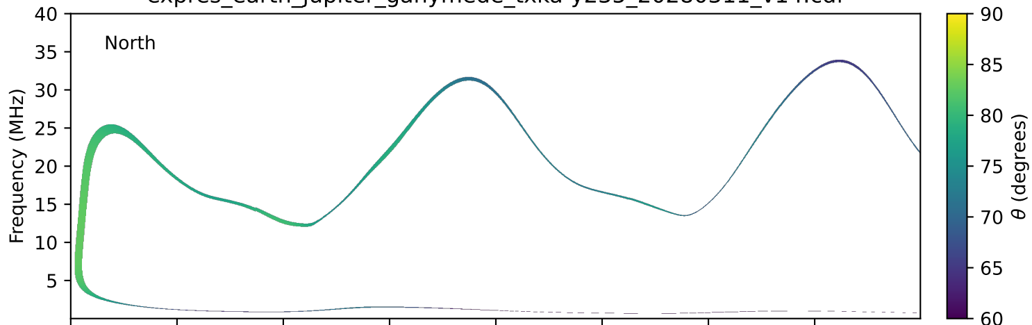
expres_earth_jupiter_ganymede_txka-y235_20280311_v14.cdf
