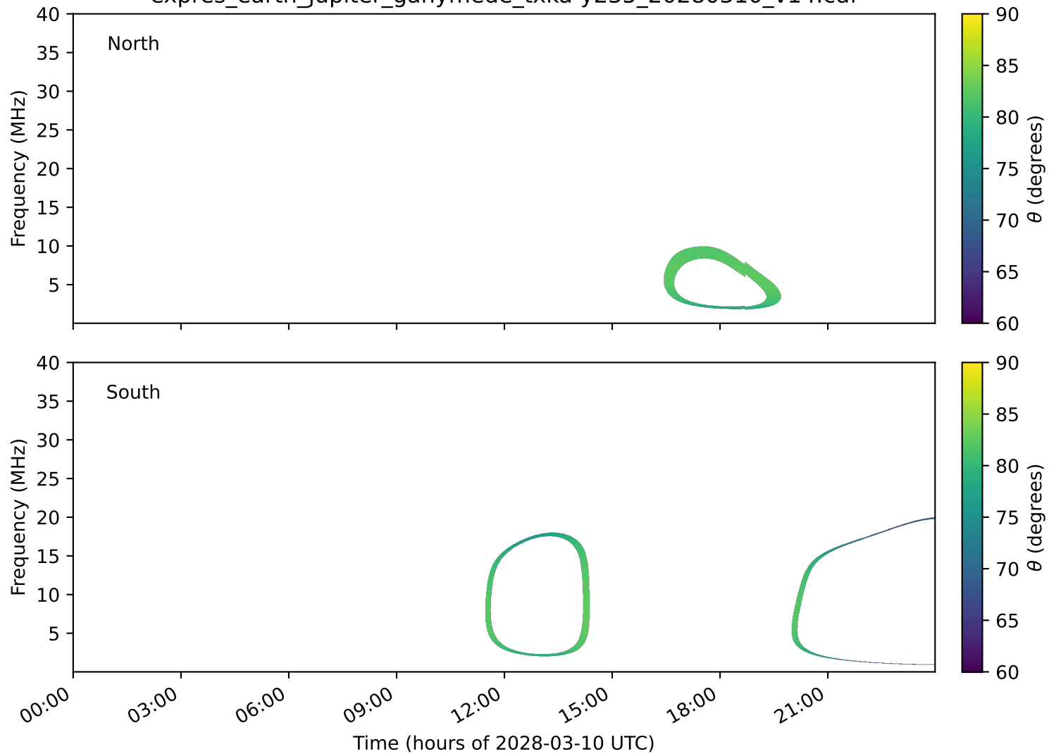
expres_earth_jupiter_ganymede_txka-y235_20280310_v14.cdf
