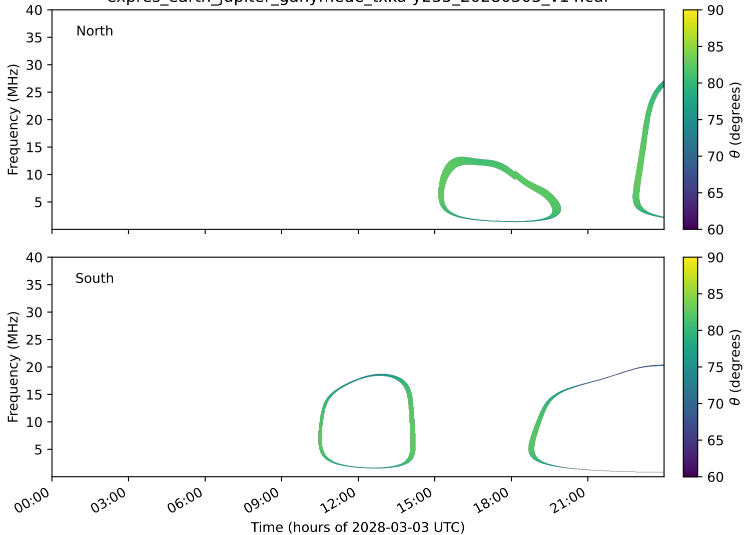
expres_earth_jupiter_ganymede_txka-y235_20280303_v14.cdf
