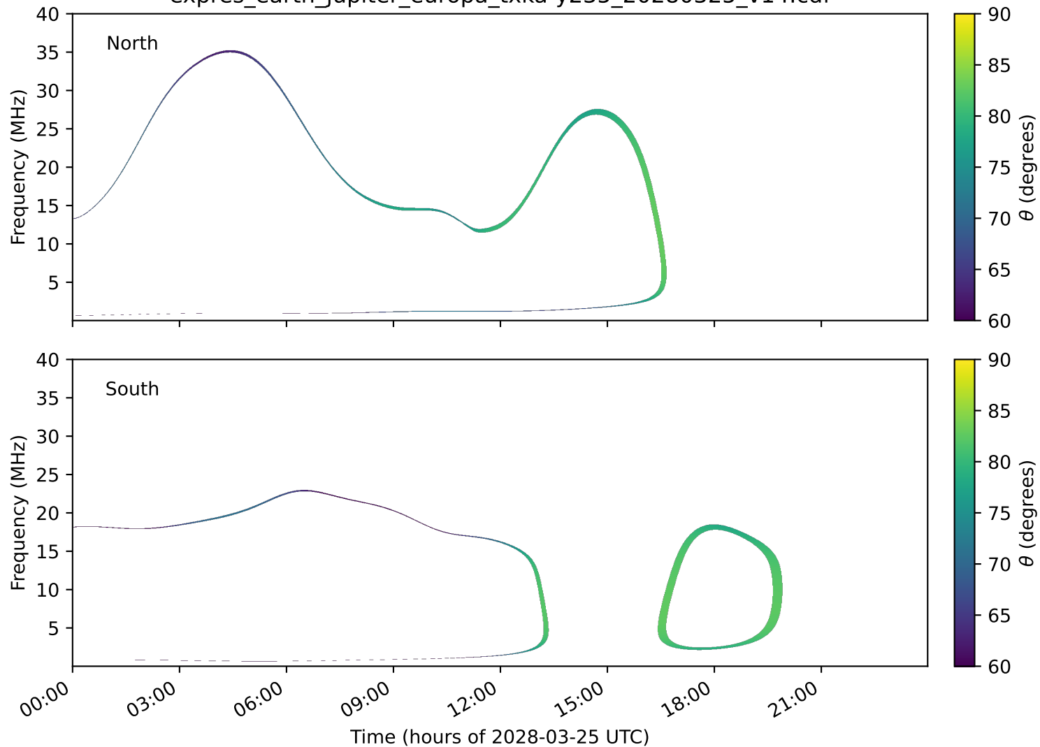
expres_earth_jupiter_europa_txka-y235_20280325_v14.cdf
