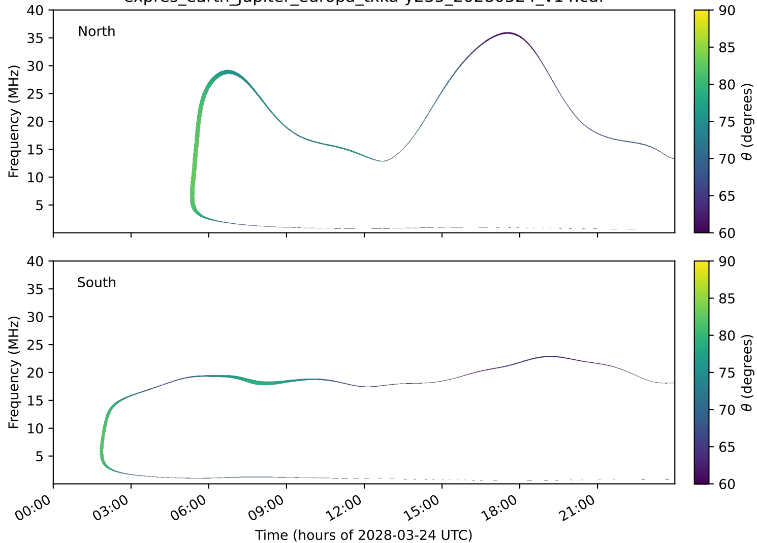
expres_earth_jupiter_europa_txka-y235_20280324_v14.cdf
