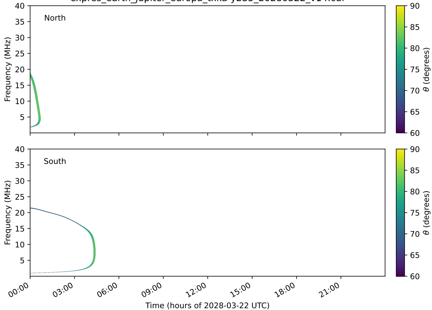
expres_earth_jupiter_europa_txka-y235_20280322_v14.cdf
