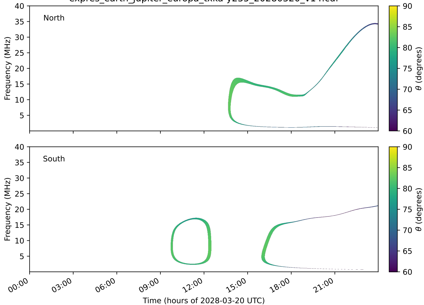
expres_earth_jupiter_europa_txka-y235_20280320_v14.cdf
