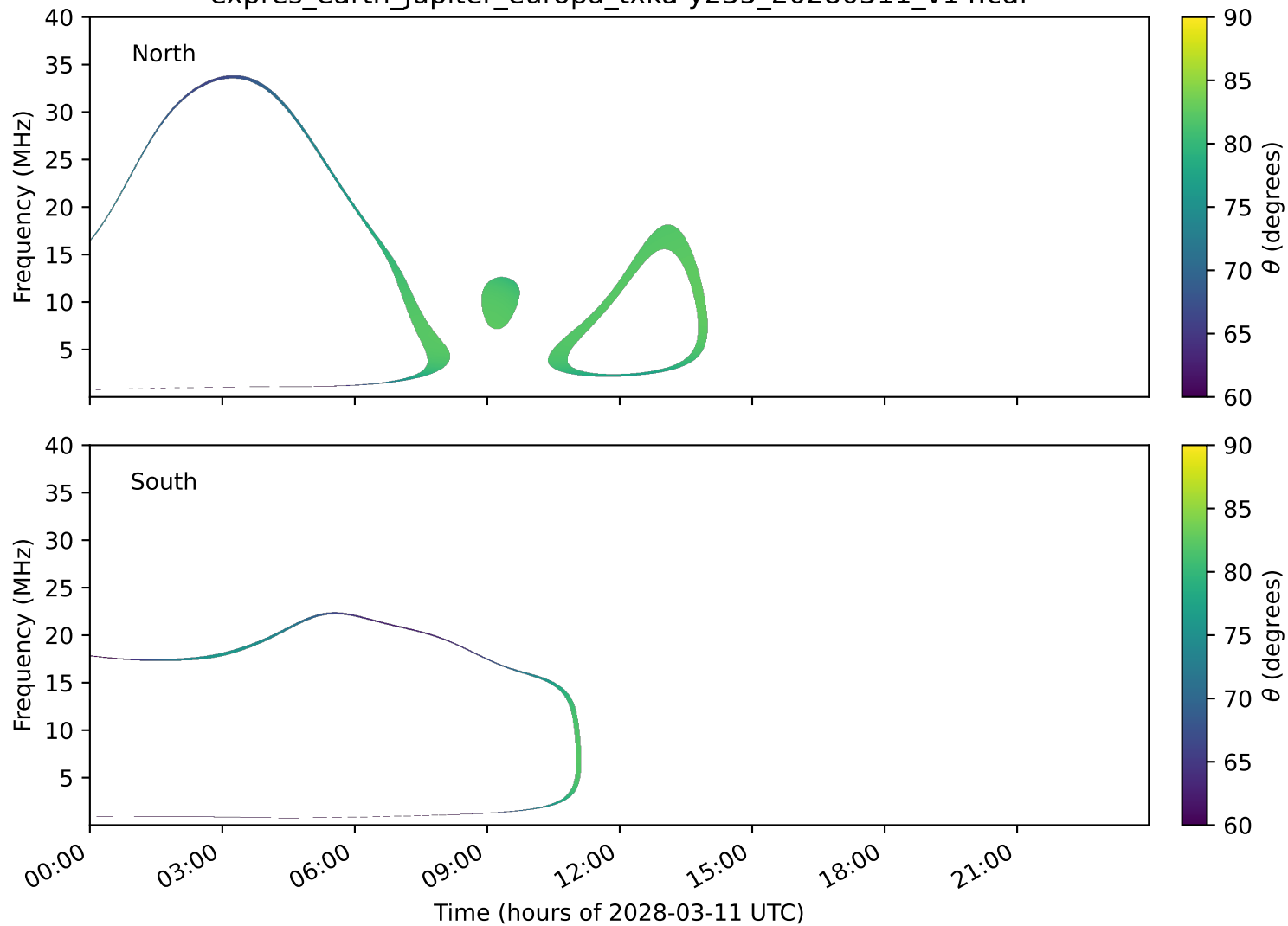
expres_earth_jupiter_europa_txka-y235_20280311_v14.cdf
