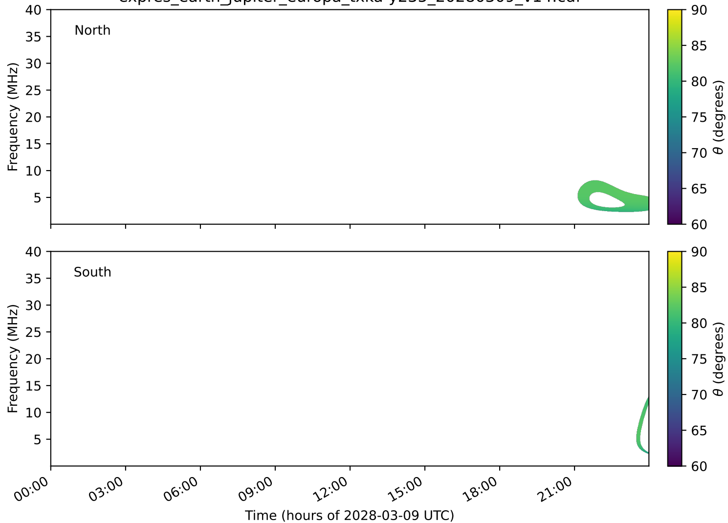
expres_earth_jupiter_europa_txka-y235_20280309_v14.cdf
