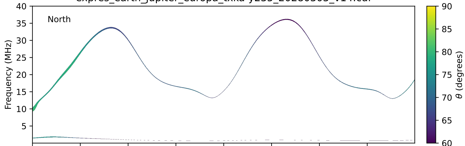
expres_earth_jupiter_europa_txka-y235_20280303_v14.cdf
