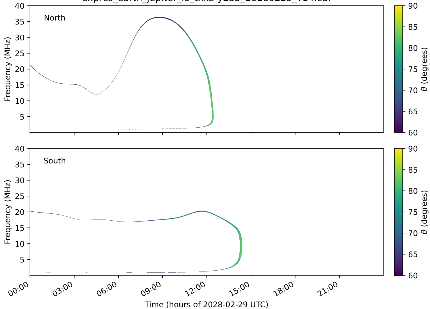
expres_earth_jupiter_io_txka-y235_20280229_v14.cdf
