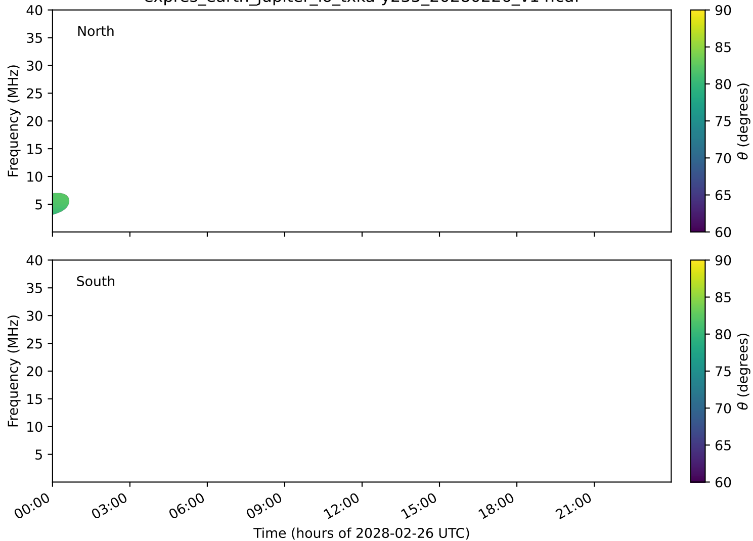
expres_earth_jupiter_io_txka-y235_20280226_v14.cdf
