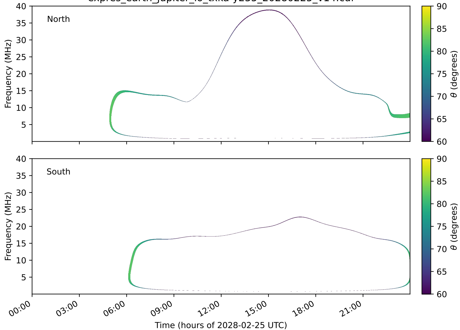
expres_earth_jupiter_io_txka-y235_20280225_v14.cdf
