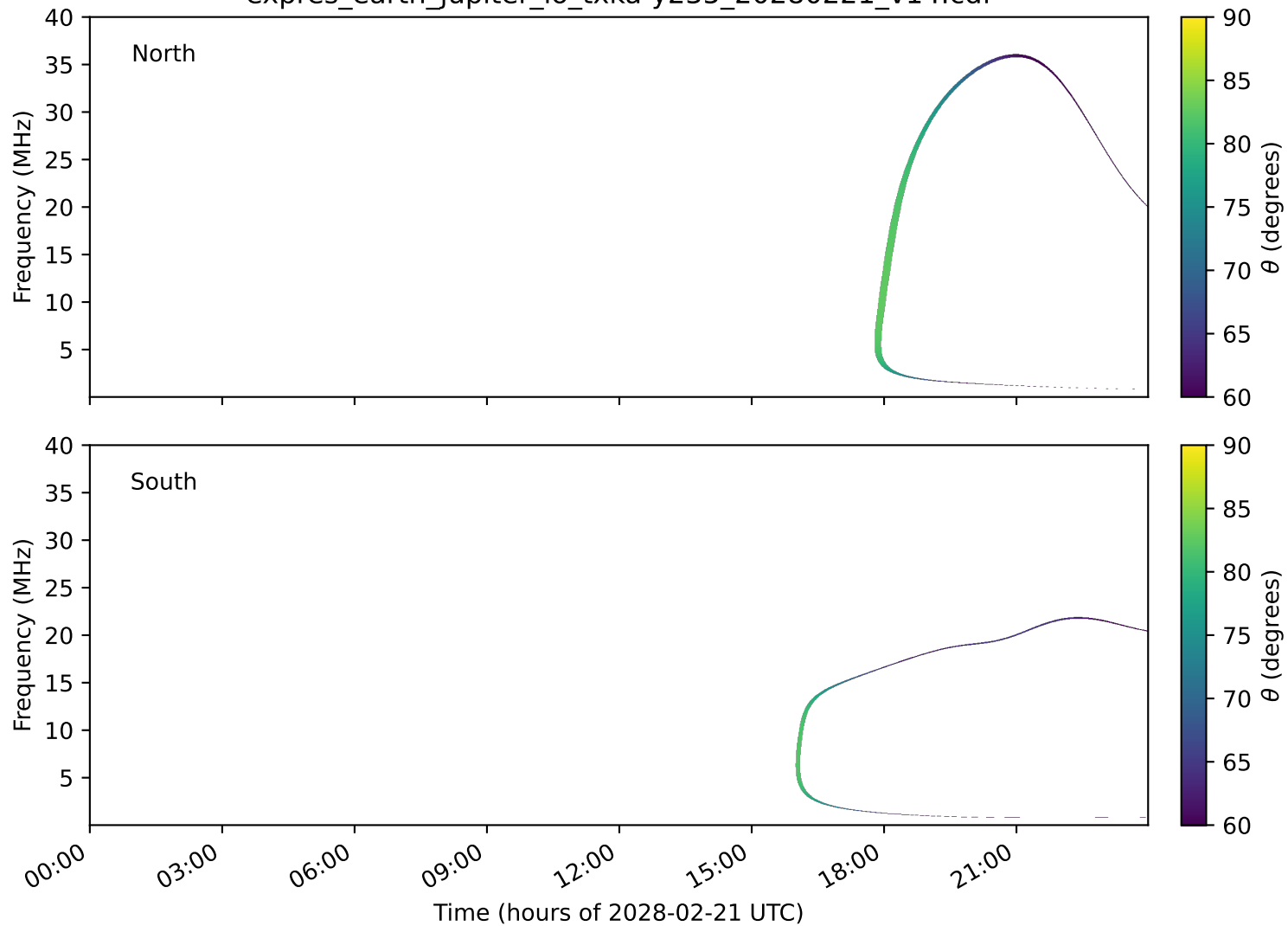
expres_earth_jupiter_io_txka-y235_20280221_v14.cdf
