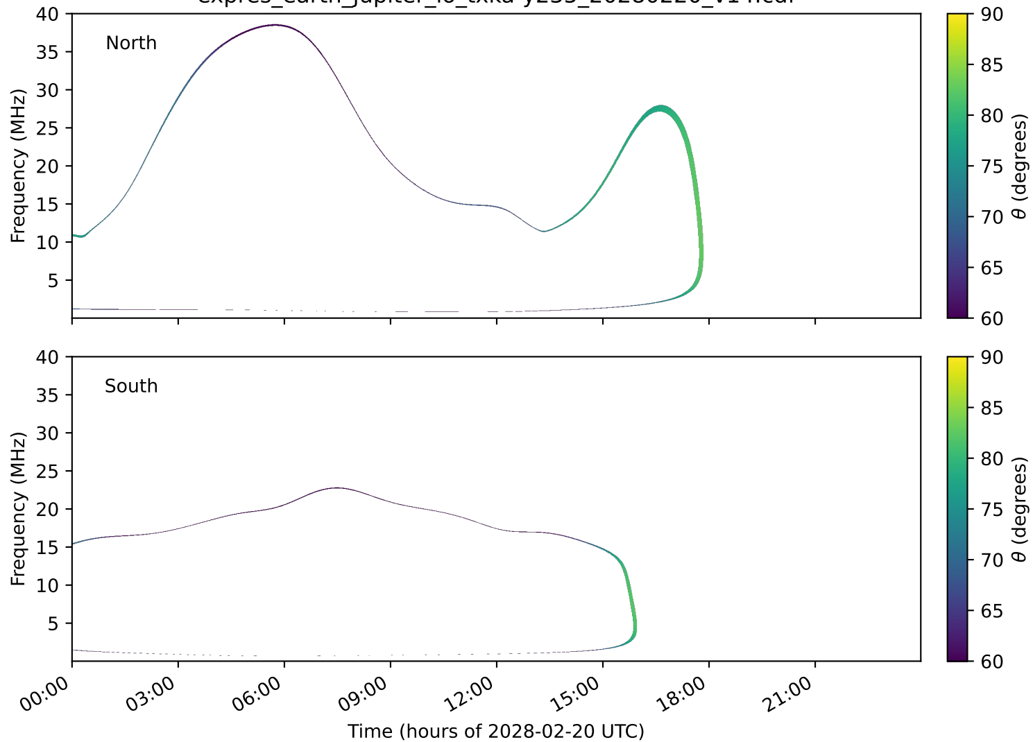
expres_earth_jupiter_io_txka-y235_20280220_v14.cdf
