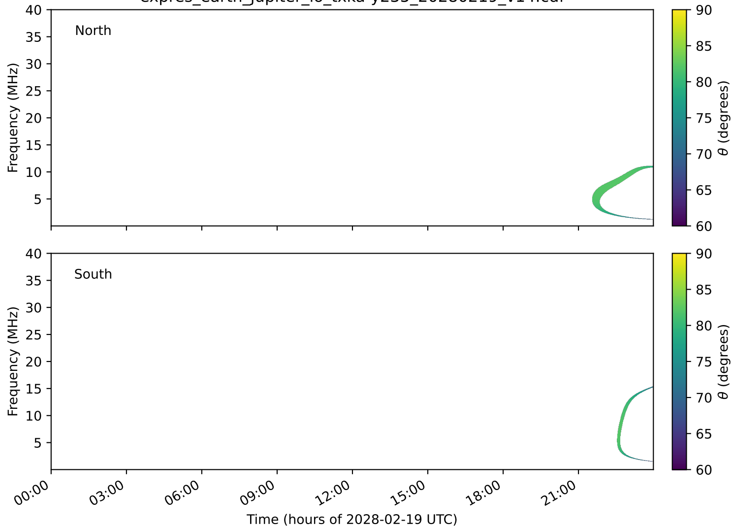
expres_earth_jupiter_io_txka-y235_20280219_v14.cdf
