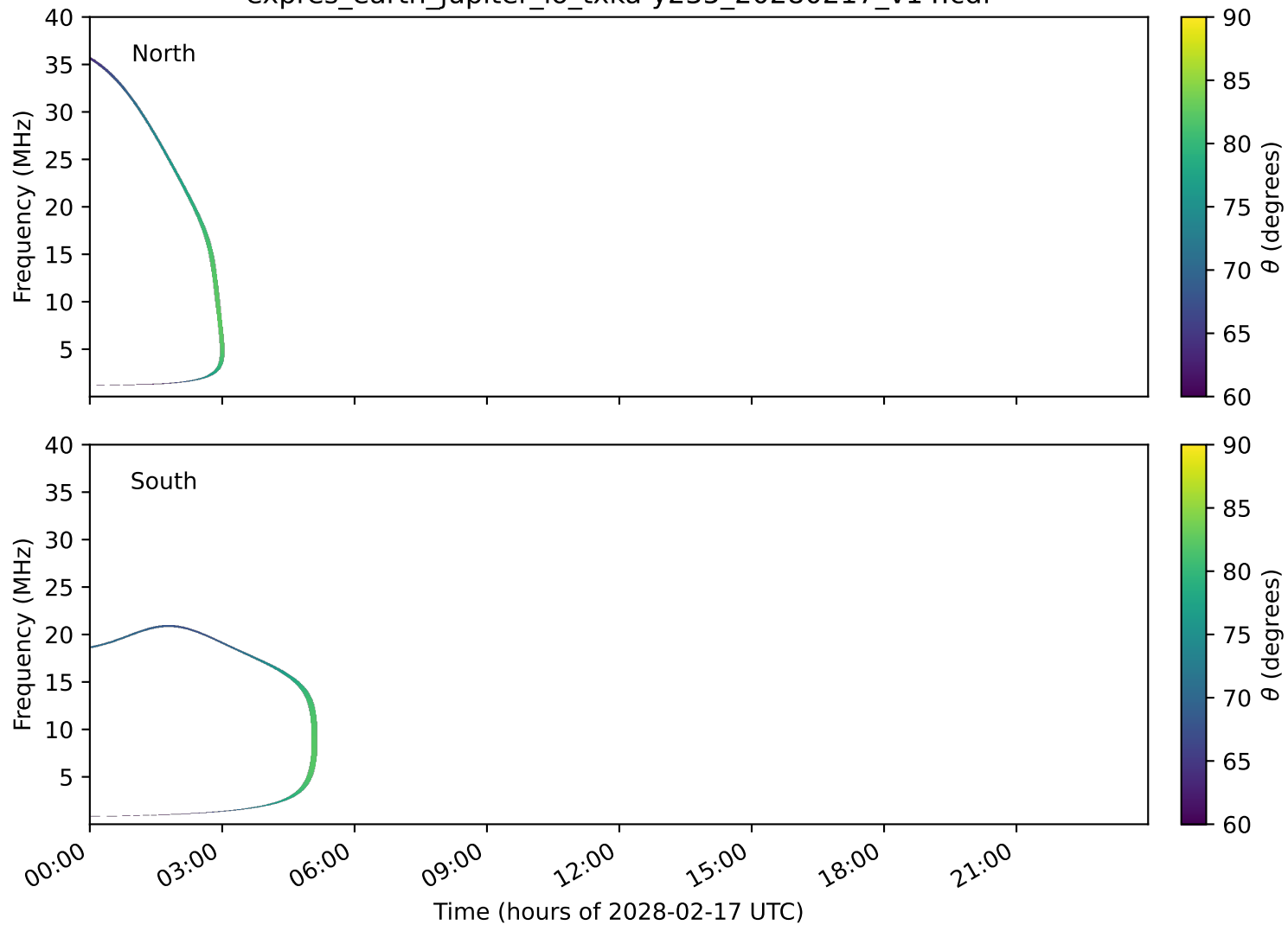
expres_earth_jupiter_io_txka-y235_20280217_v14.cdf
