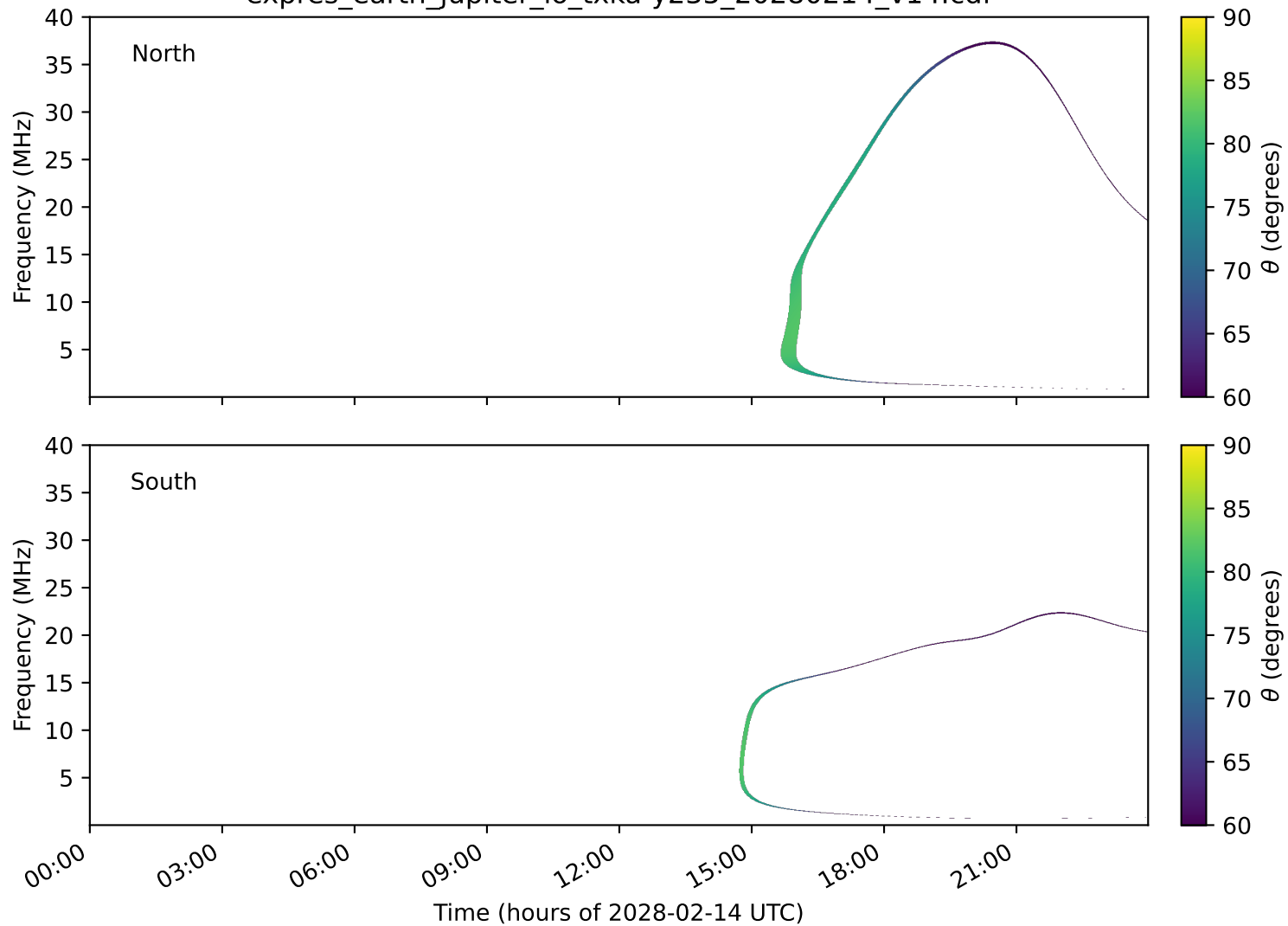
expres_earth_jupiter_io_txka-y235_20280214_v14.cdf
