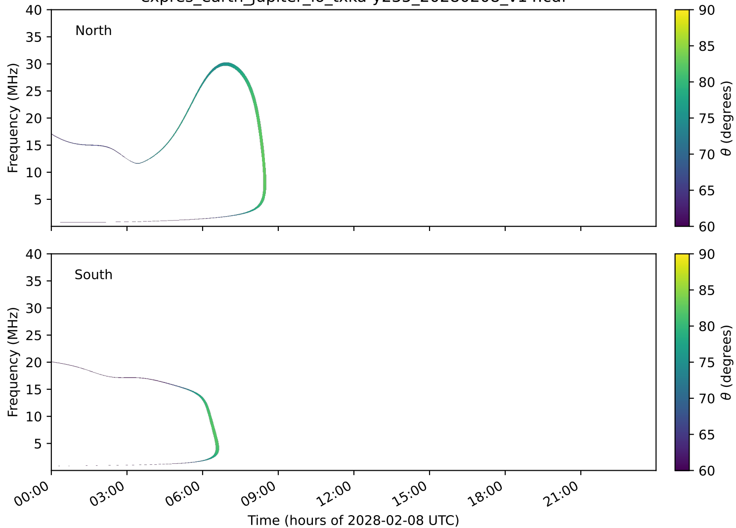
expres_earth_jupiter_io_txka-y235_20280208_v14.cdf
