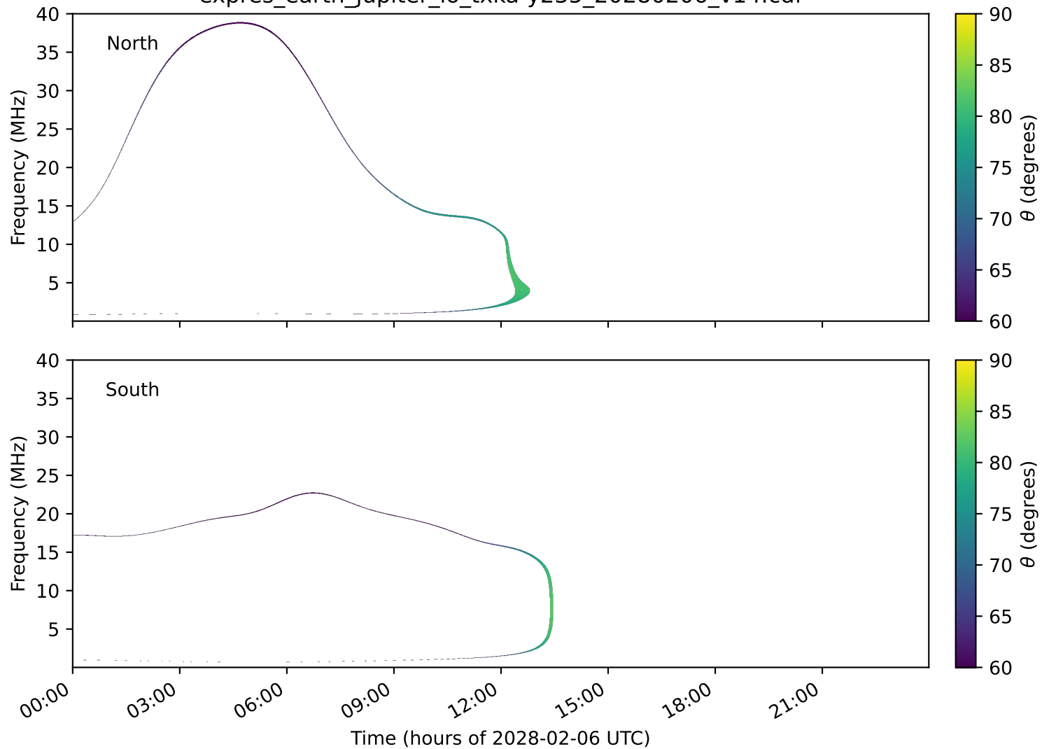
expres_earth_jupiter_io_txka-y235_20280206_v14.cdf
