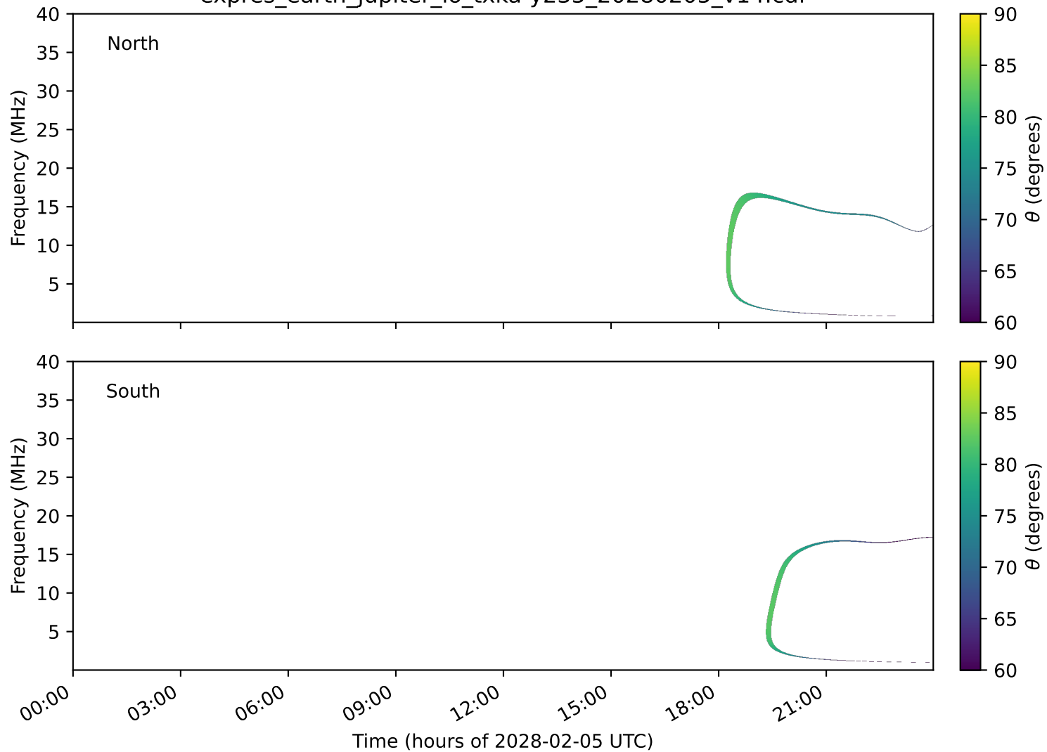
expres_earth_jupiter_io_txka-y235_20280205_v14.cdf
