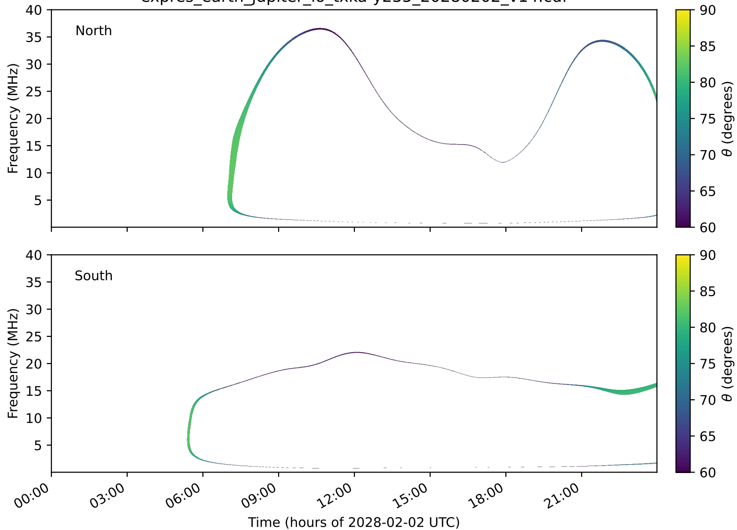
expres_earth_jupiter_io_txka-y235_20280202_v14.cdf
