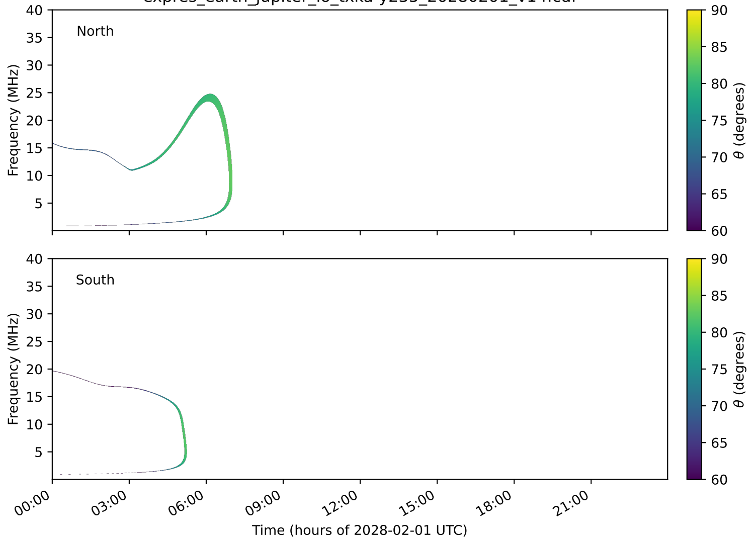
expres_earth_jupiter_io_txka-y235_20280201_v14.cdf
