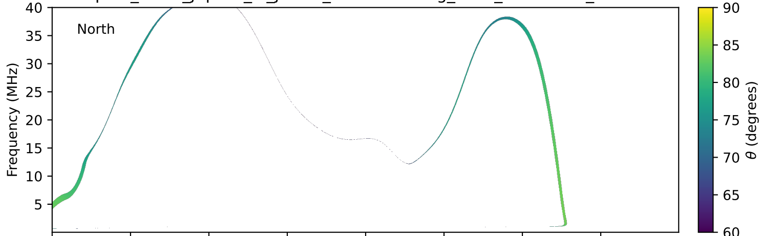
expres_earth_jupiter_io_jrm33_lossc-wid1deg_3kev_20280227_v11.cdf
