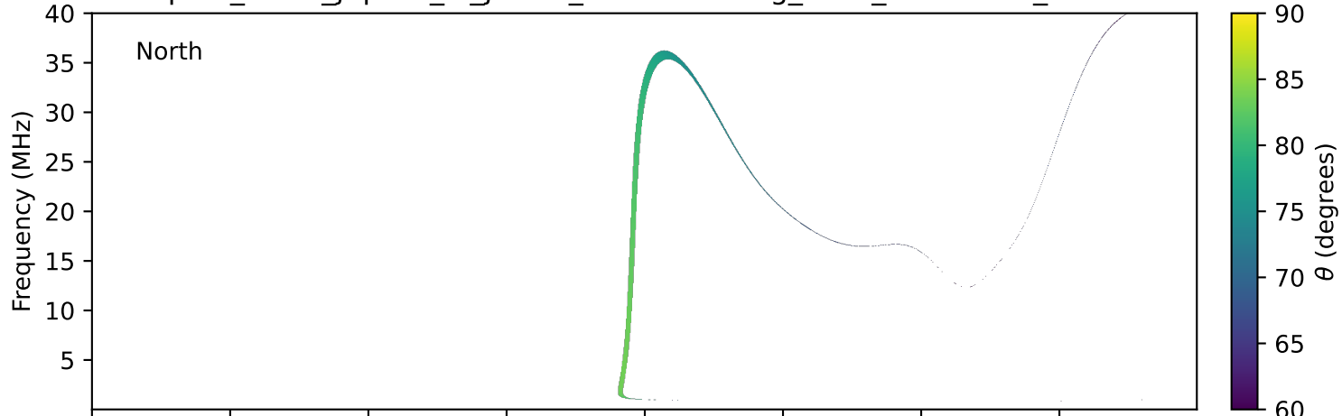
expres_earth_jupiter_io_jrm33_lossc-wid1deg_3kev_20280223_v11.cdf
