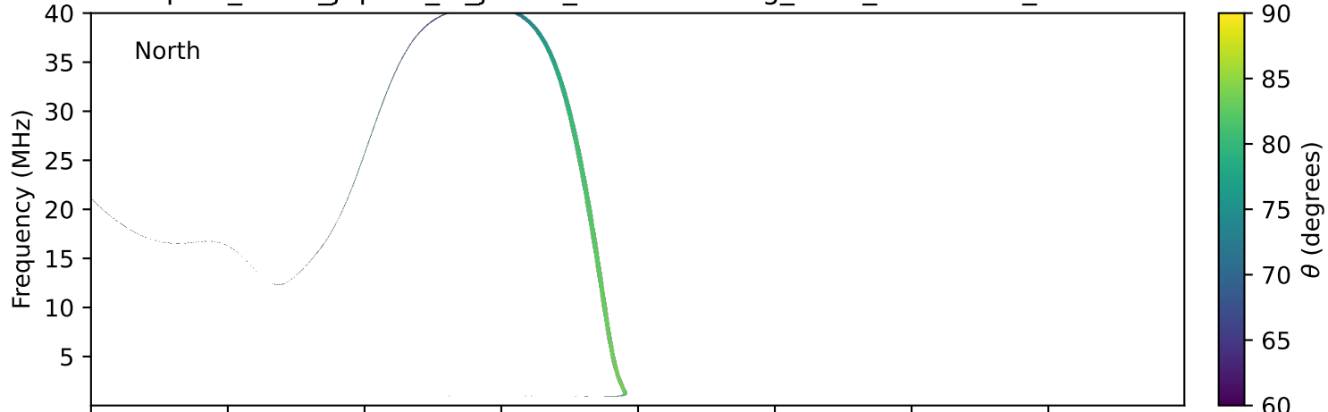
expres_earth_jupiter_io_jrm33_lossc-wid1deg_3kev_20280222_v11.cdf
