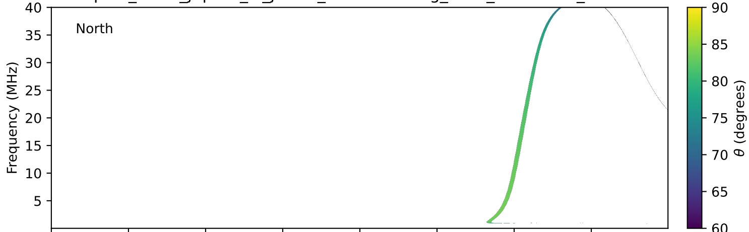
expres_earth_jupiter_io_jrm33_lossc-wid1deg_3kev_20280221_v11.cdf
