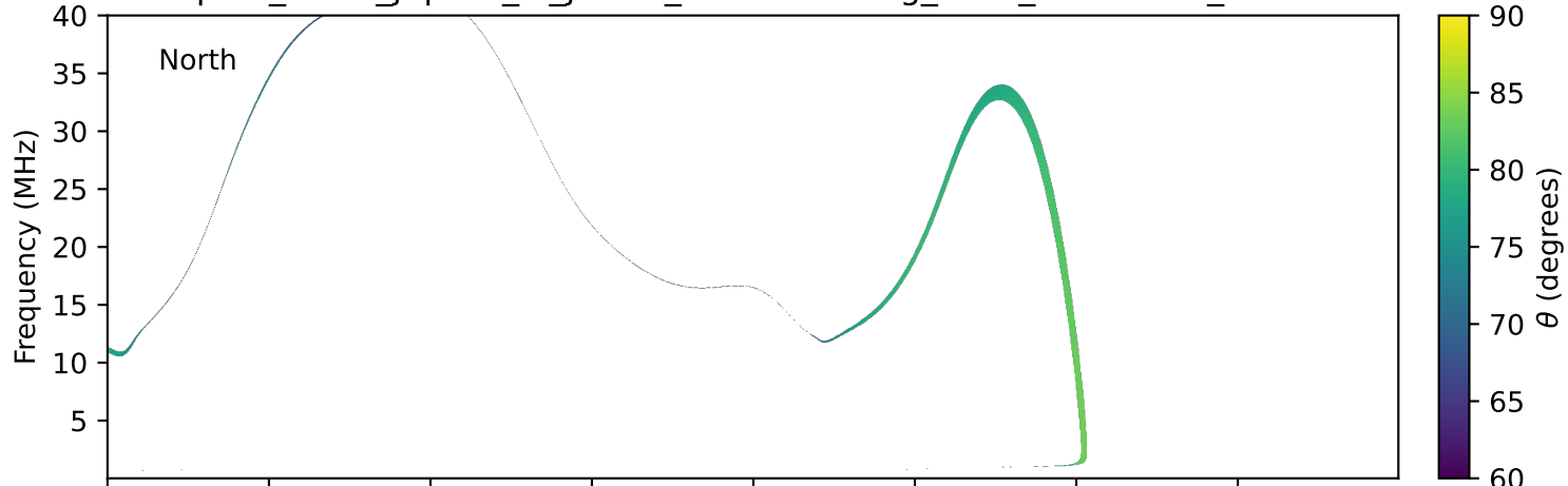
expres_earth_jupiter_io_jrm33_lossc-wid1deg_3kev_20280220_v11.cdf
