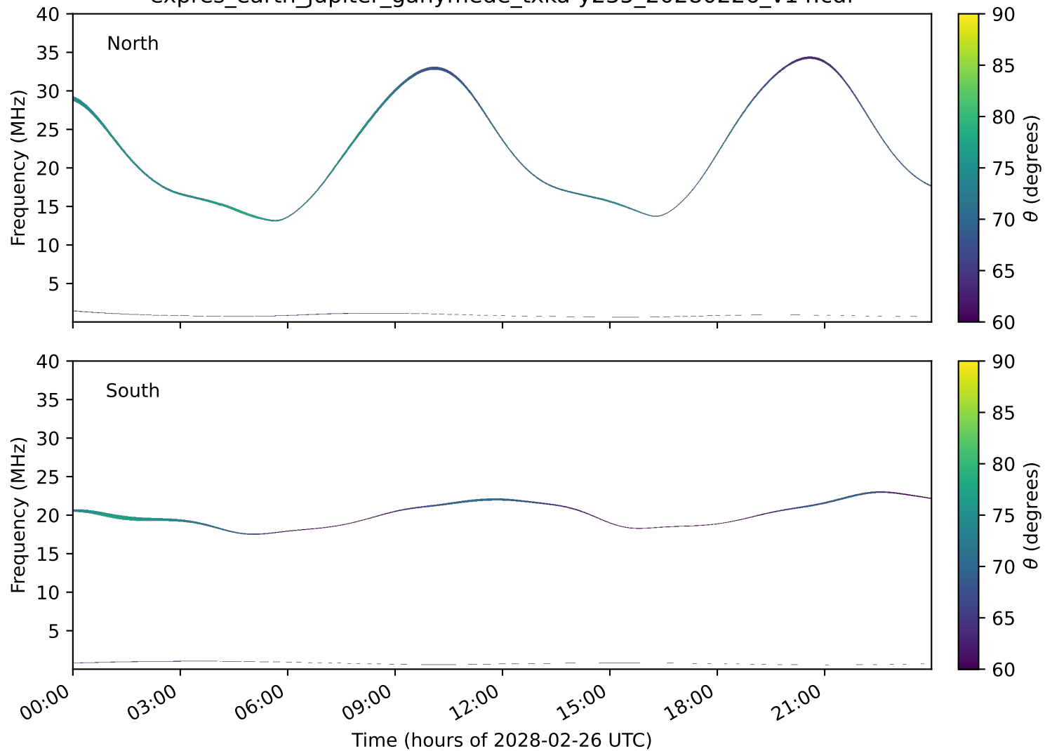
expres_earth_jupiter_ganymede_txka-y235_20280226_v14.cdf
