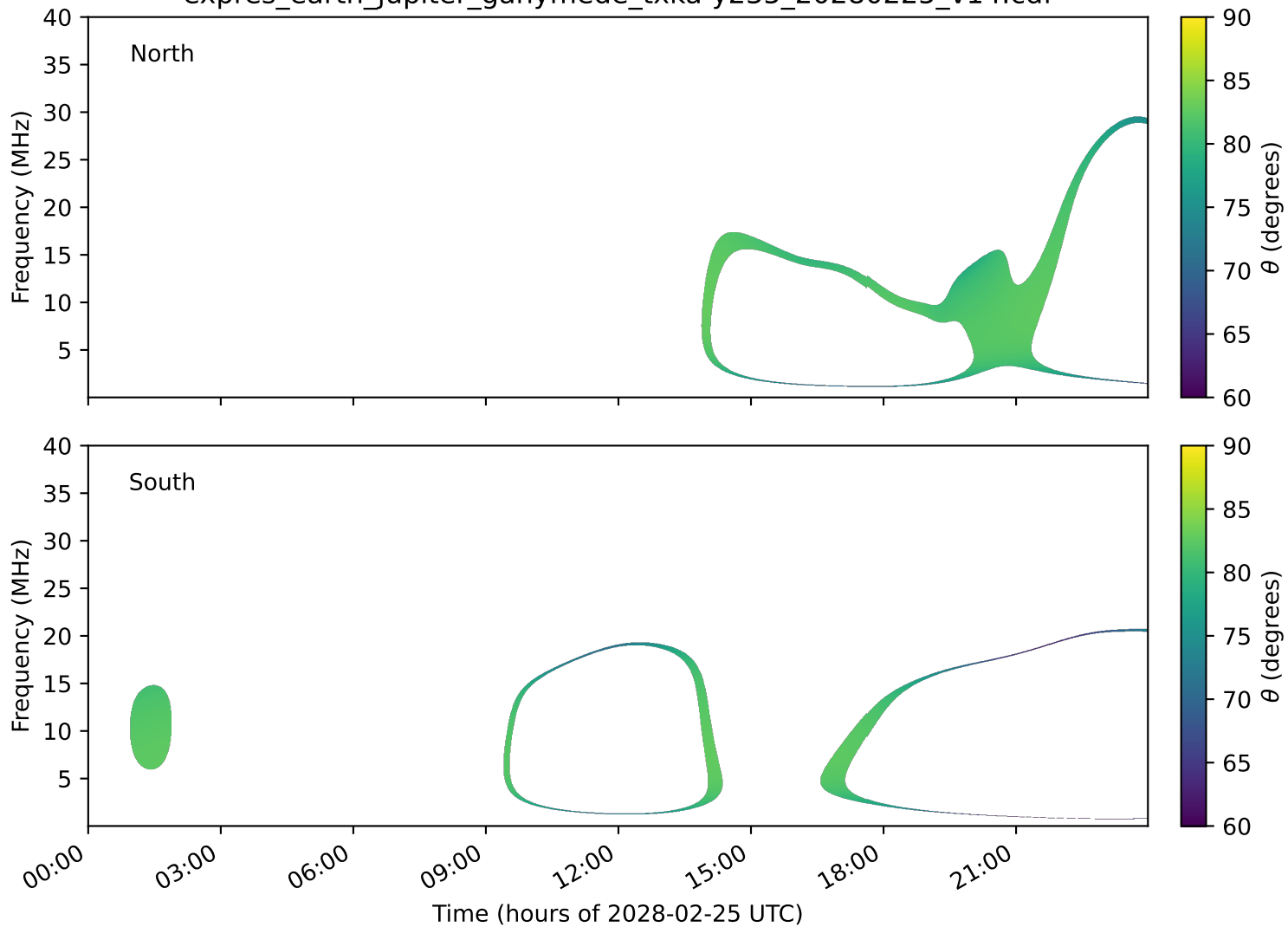
expres_earth_jupiter_ganymede_txka-y235_20280225_v14.cdf
