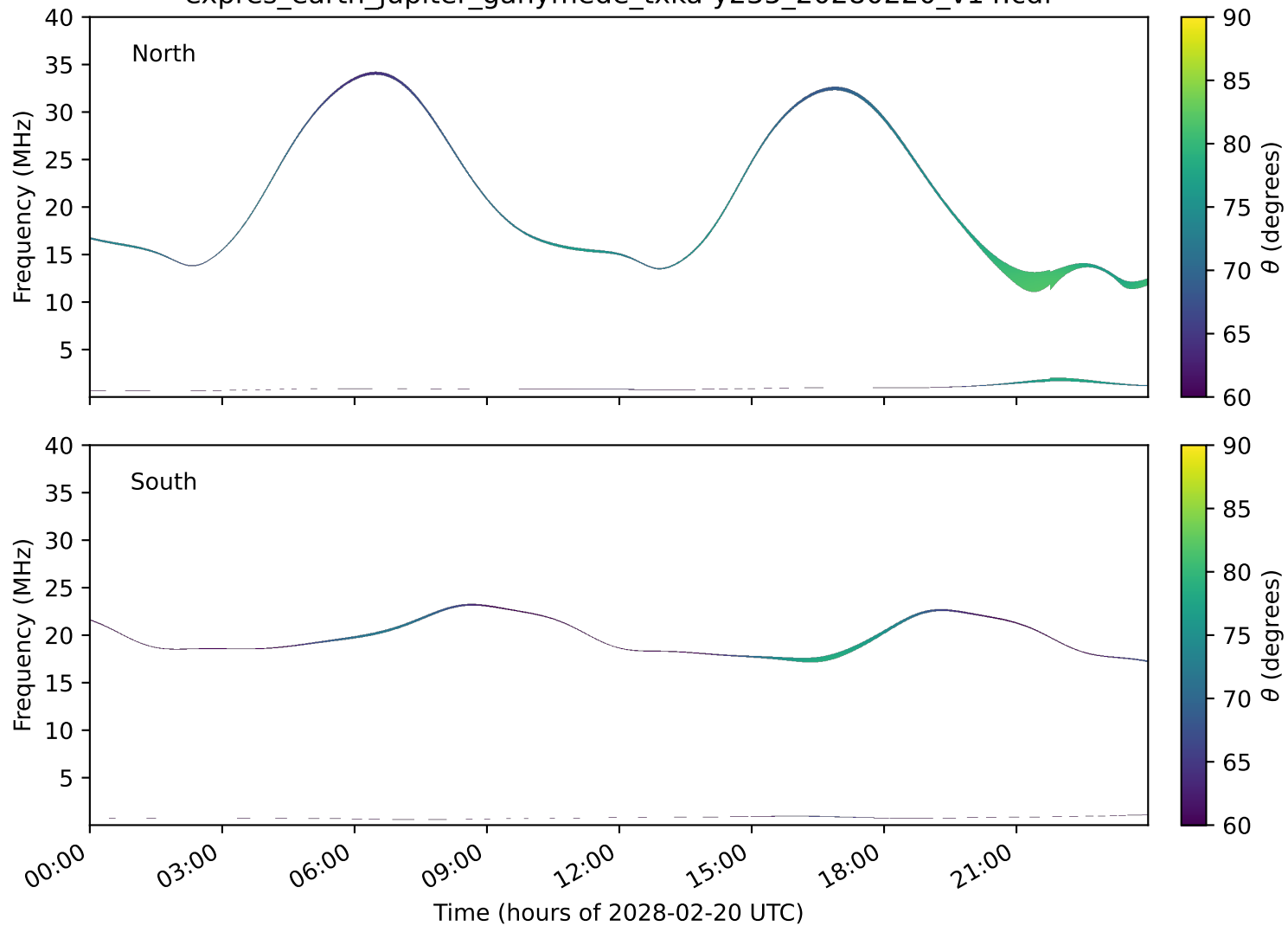
expres_earth_jupiter_ganymede_txka-y235_20280220_v14.cdf
