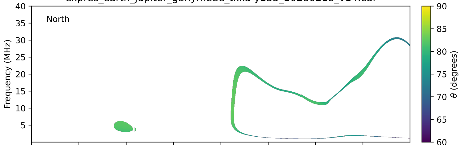
expres_earth_jupiter_ganymede_txka-y235_20280218_v14.cdf
