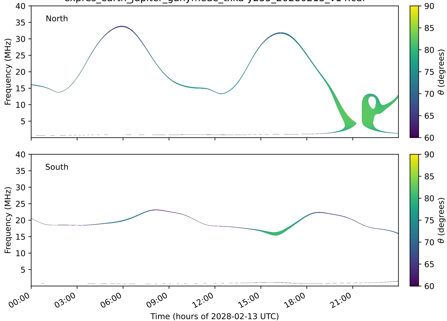
expres_earth_jupiter_ganymede_txka-y235_20280213_v14.cdf
