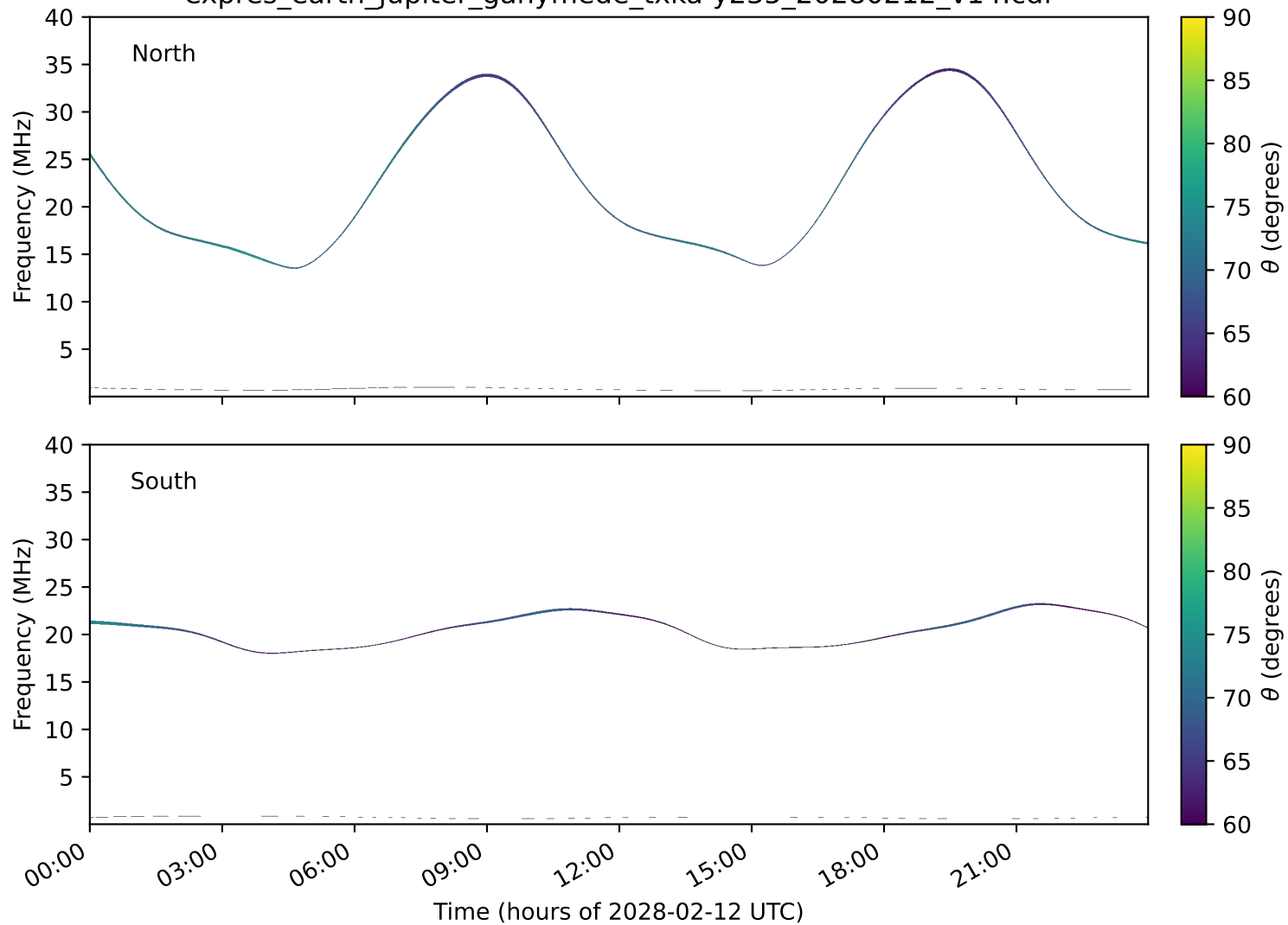
expres_earth_jupiter_ganymede_txka-y235_20280212_v14.cdf
