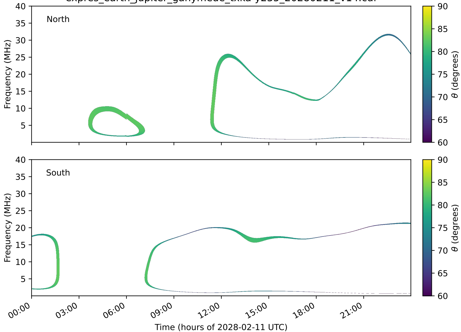
expres_earth_jupiter_ganymede_txka-y235_20280211_v14.cdf
