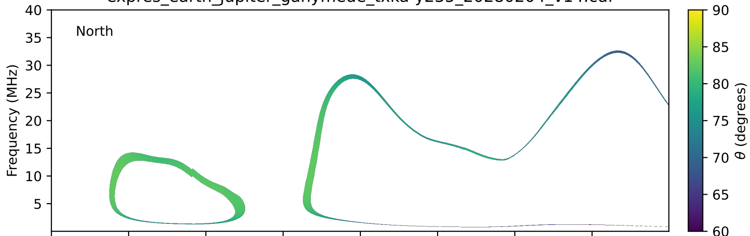
expres_earth_jupiter_ganymede_txka-y235_20280204_v14.cdf
