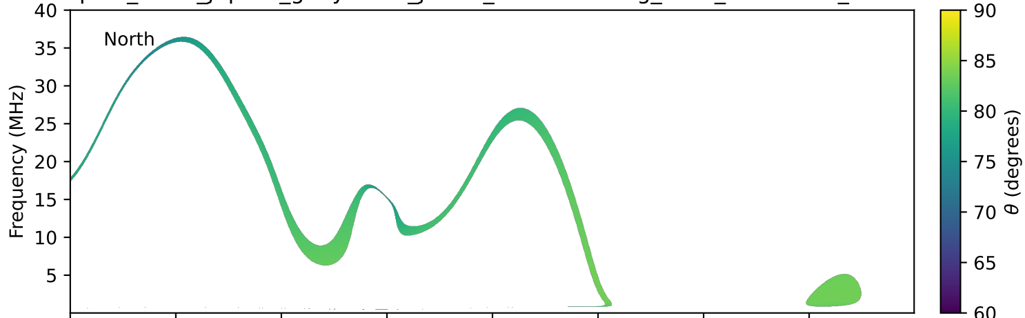
expres_earth_jupiter_ganymede_jrm33_lossc-wid1deg_3kev_20280221_v11.cdf
