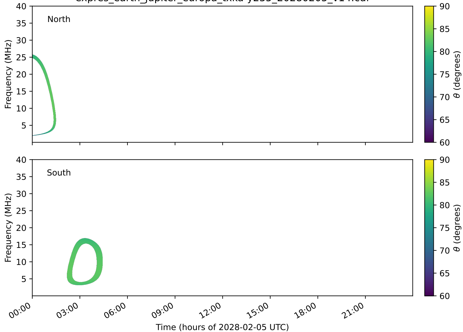
expres_earth_jupiter_europa_txka-y235_20280205_v14.cdf
