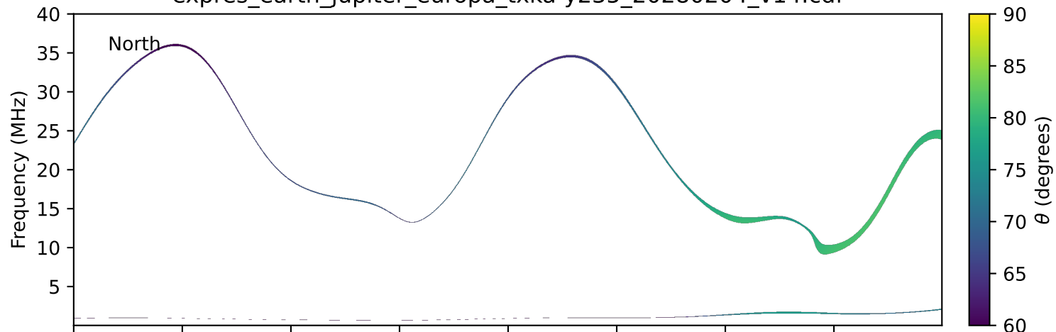
expres_earth_jupiter_europa_txka-y235_20280204_v14.cdf
