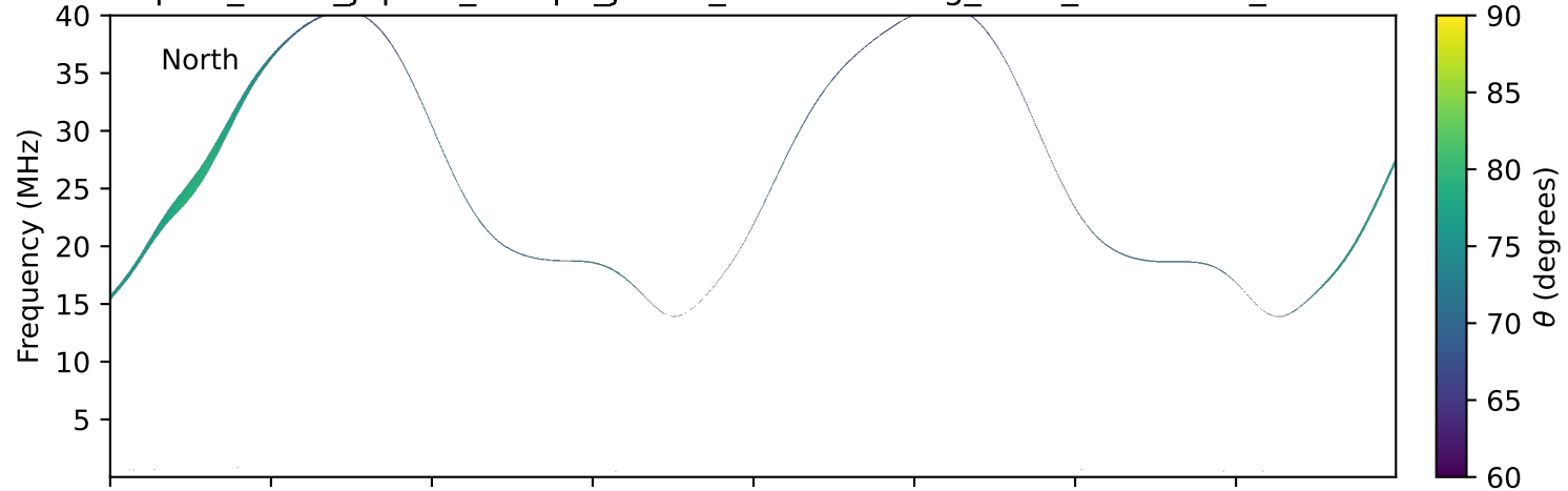
expres_earth_jupiter_europa_jrm33_lossc-wid1deg_3kev_20280225_v11.cdf
