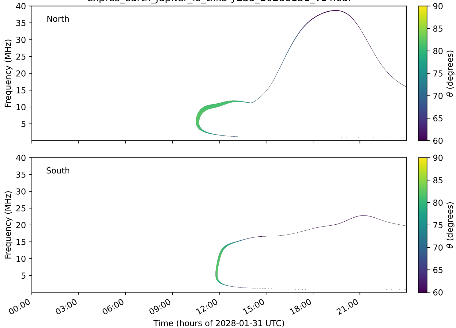
expres_earth_jupiter_io_txka-y235_20280131_v14.cdf
