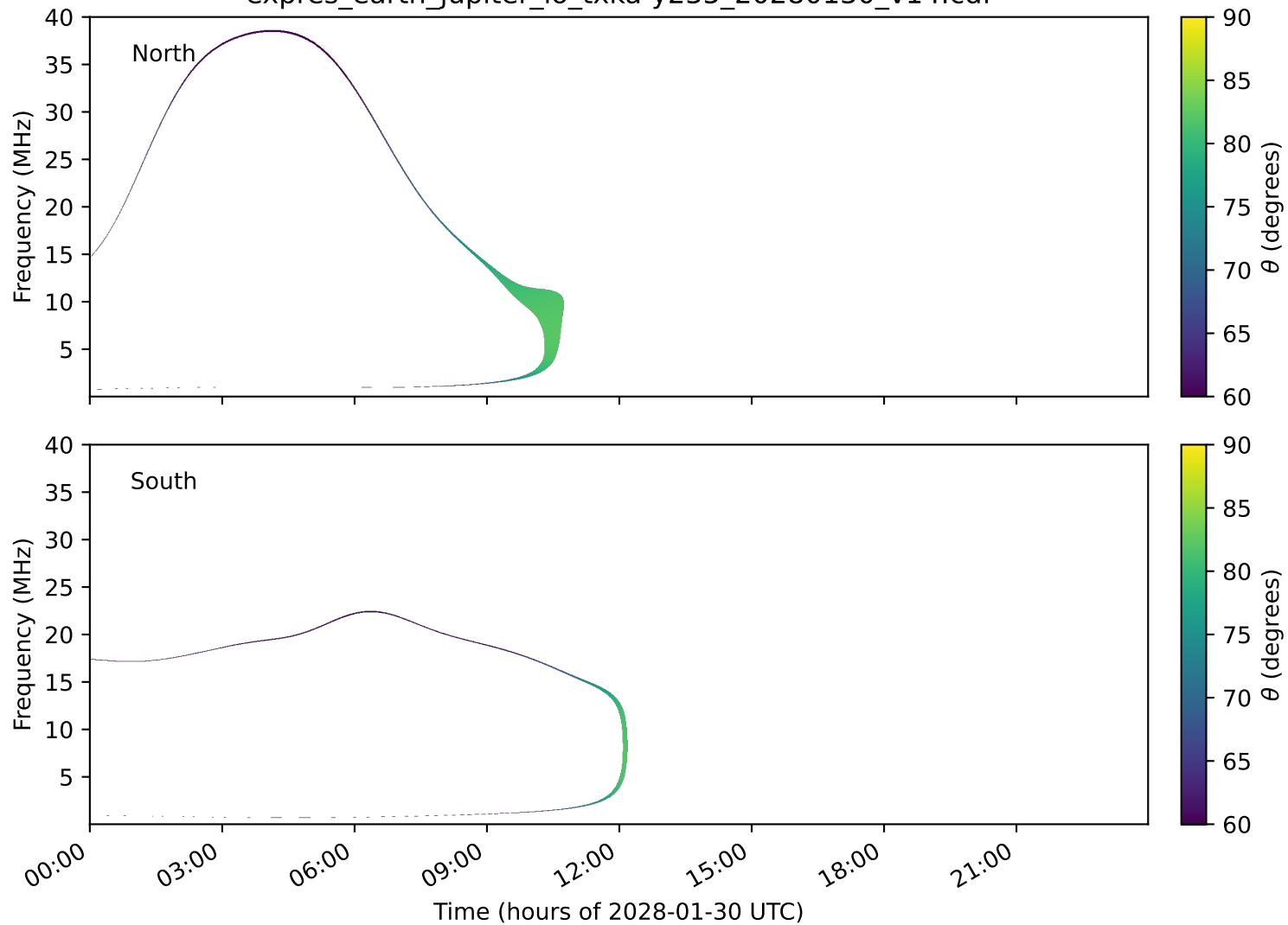
expres_earth_jupiter_io_txka-y235_20280130_v14.cdf
