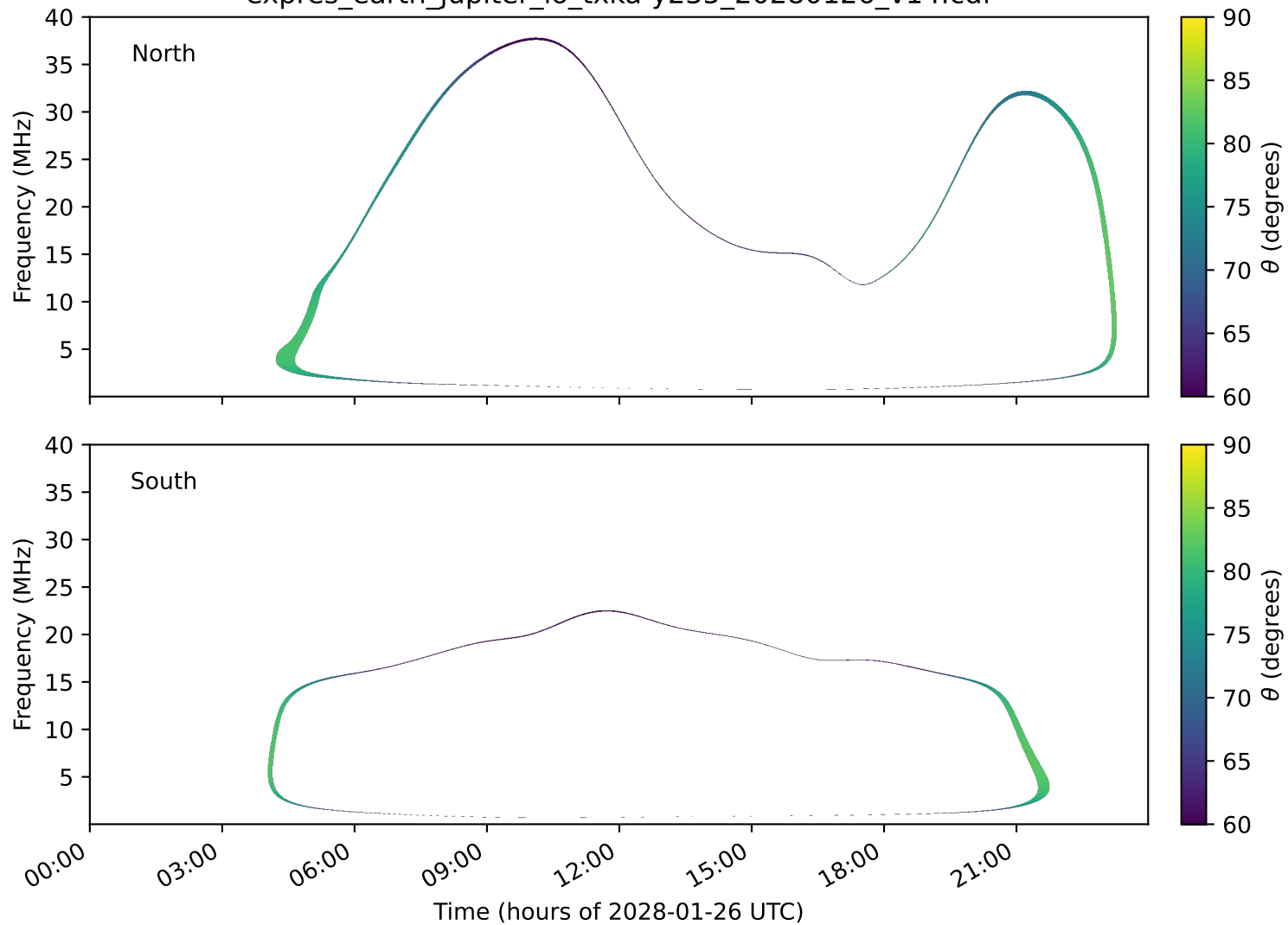
expres_earth_jupiter_io_txka-y235_20280126_v14.cdf
