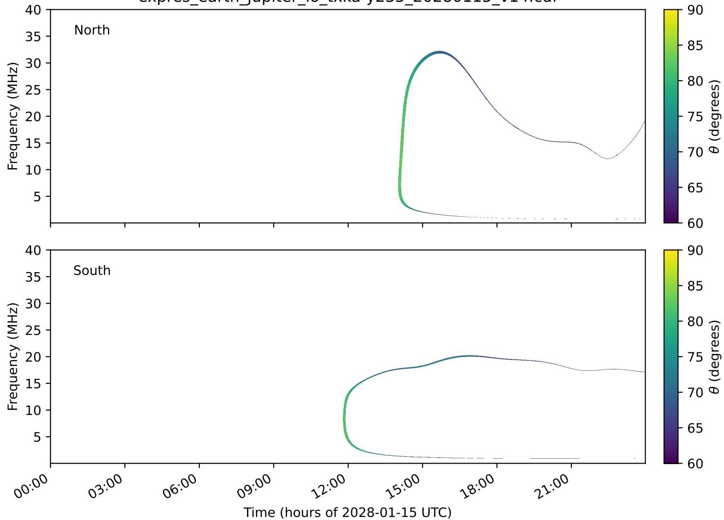
expres_earth_jupiter_io_txka-y235_20280115_v14.cdf
