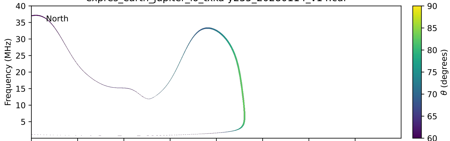
expres_earth_jupiter_io_txka-y235_20280114_v14.cdf
